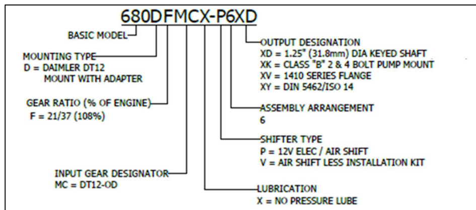
Figure 19: Model Chart for the Chelsea 680 PTO and the DT12-OD (OVX).
