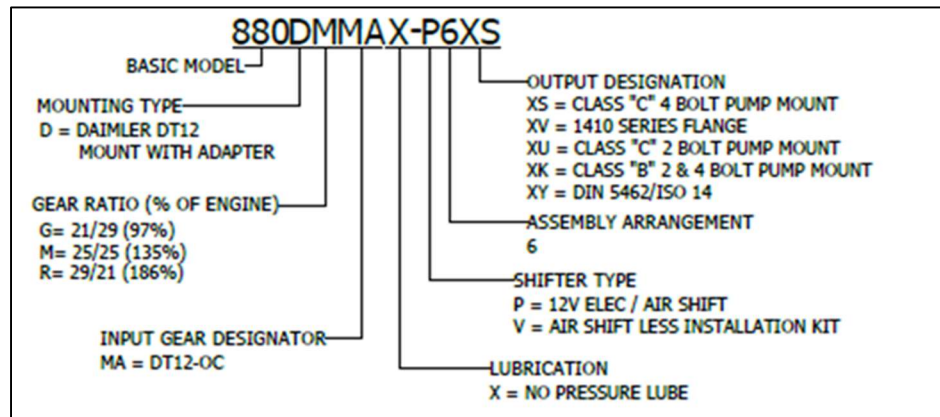
Figure 15: Model Chart for the Chelsea 880 PTO and the DT12-OC (OHE & OV).
