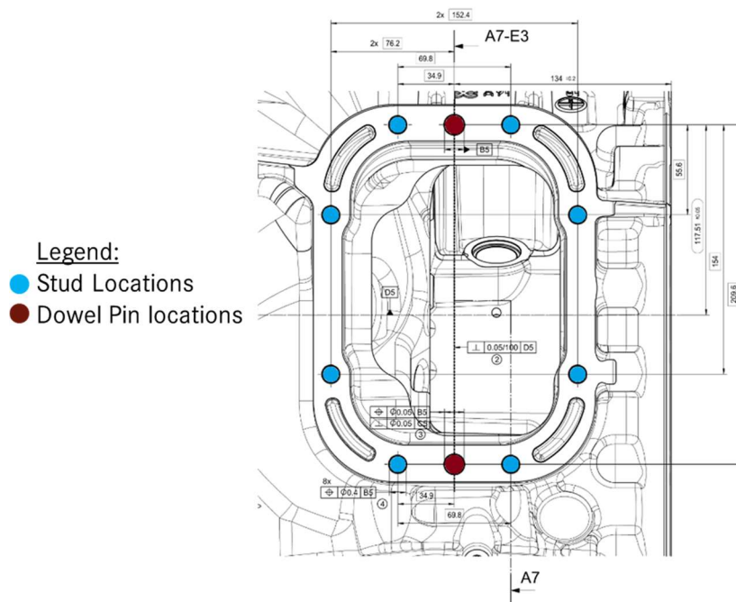
Figure 27: Stud and dowel pin installation locations
