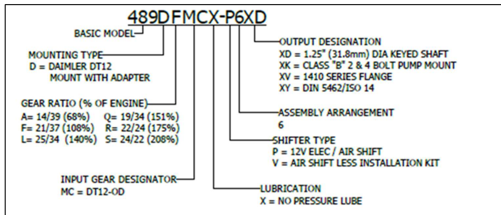
Figure 22: Model Chart for the Chelsea 489 PTO and the DT12-OD (OVX).
