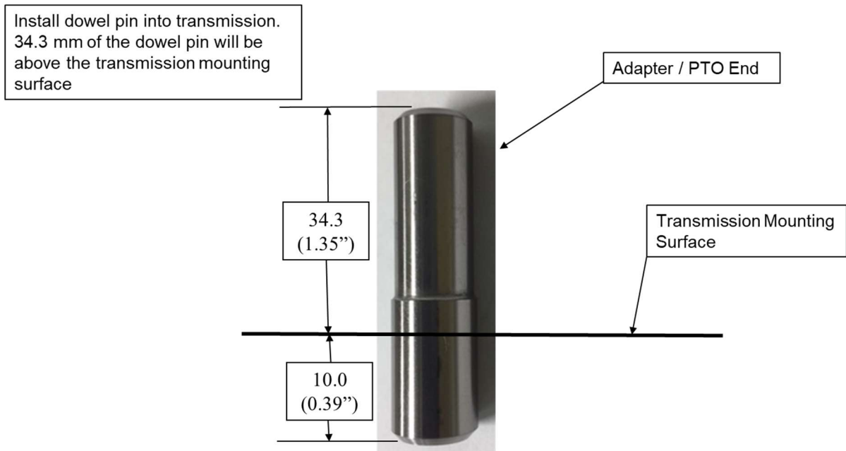
Figure 26: Stud installation information
