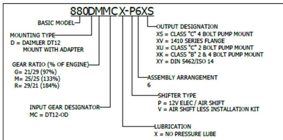
Figure 16: Model Chart for the Chelsea 880 PTO and the DT12-OD (OVX).
