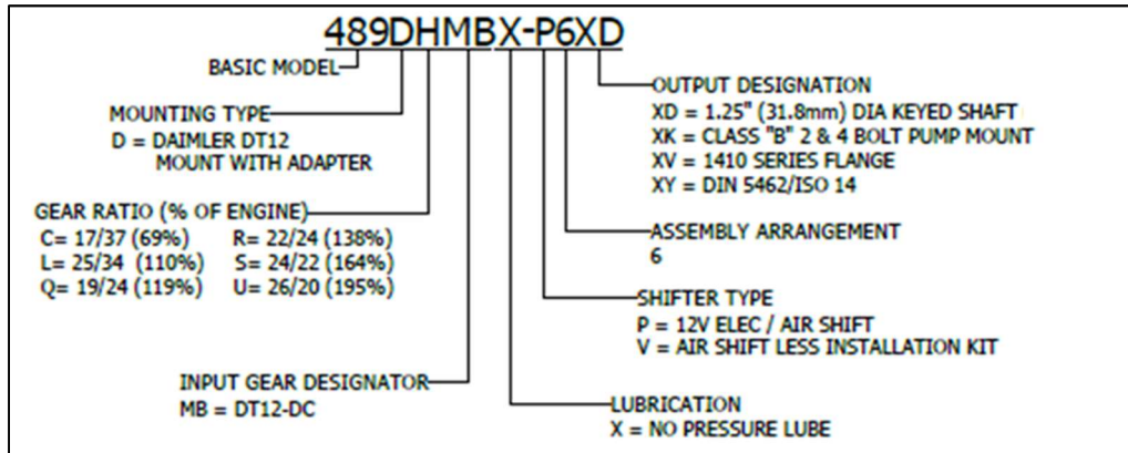
Figure 20: Model Chart for the Chelsea 489 PTO and the DT12-DC (DHE & DV).
