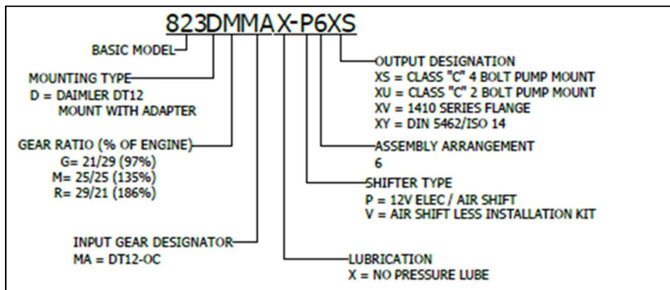
Figure 12: Model Chart for the Chelsea 823 PTO and the DT12-OC (OHE & OV).
