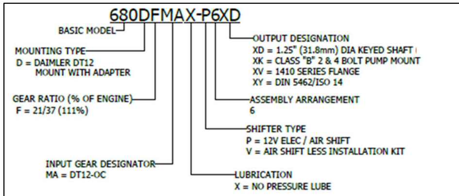
Figure 18: Model Chart for the Chelsea 680 PTO and the DT12-OC (OHE & OV).
