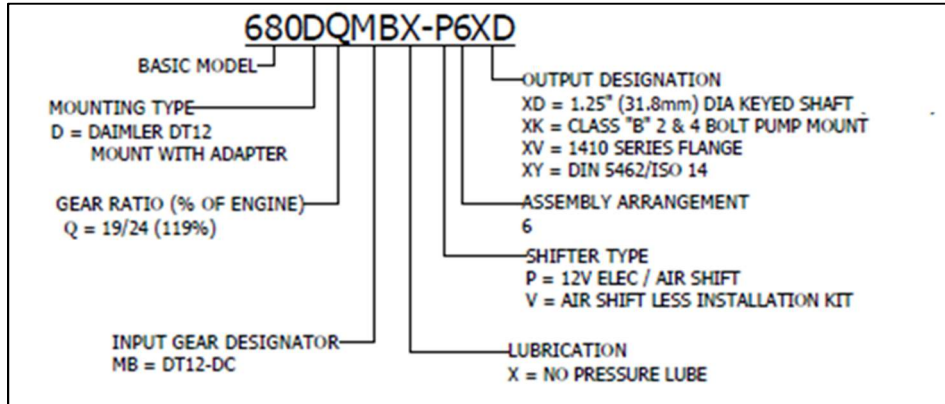
Figure 17: Model Chart for the Chelsea 680 PTO and the DT12-DC (DHE & DV)
