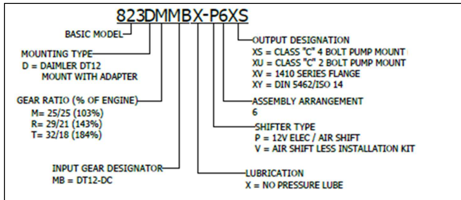
Figure 11: Model Chart for the Chelsea 823 PTO and the DT12-DC (DHE & DV).
