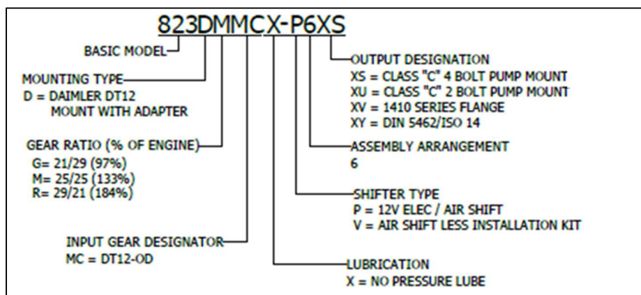
Figure 13: Model Chart for the Chelsea 823 PTO and the DT12-OD (OVX).
