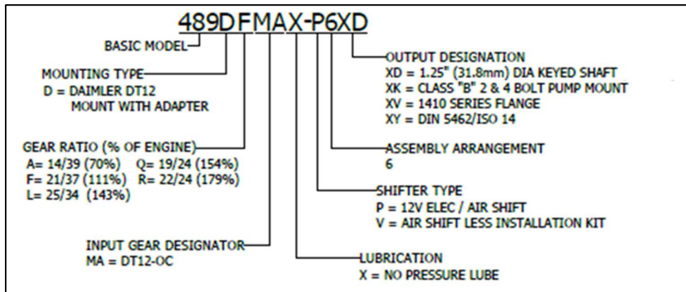
Figure 21: Model Chart for the Chelsea 489 PTO and the DT12-OC (OHE & OV).
