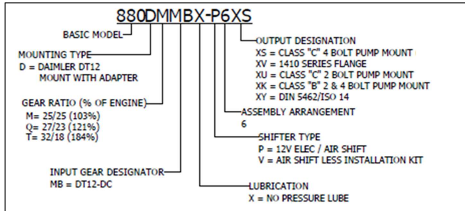
Figure 14: Model Chart for the Chelsea 880 PTO and the DT12-DC (DHE & DV).
